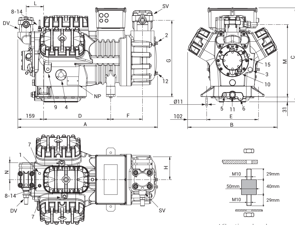
Vibration absorber
