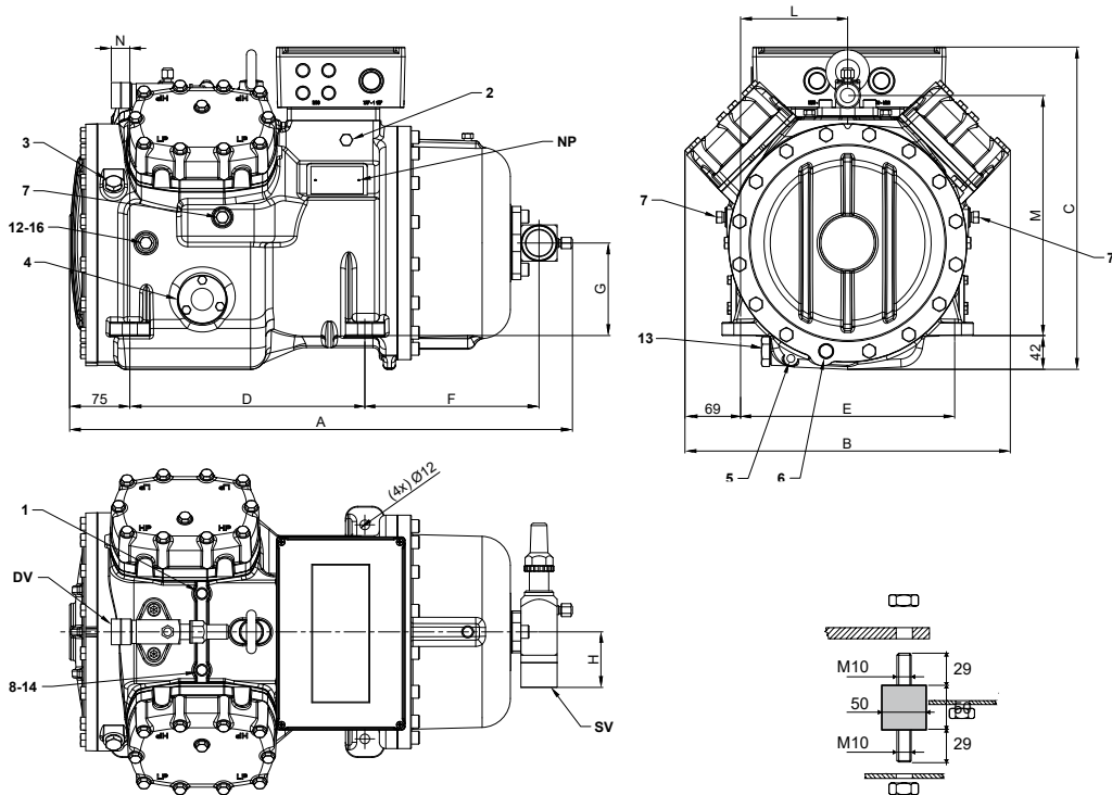
Vibration absorber
