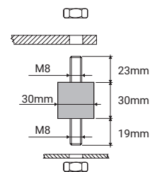
Vibration absorber
