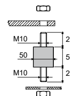
Vibration absorber
